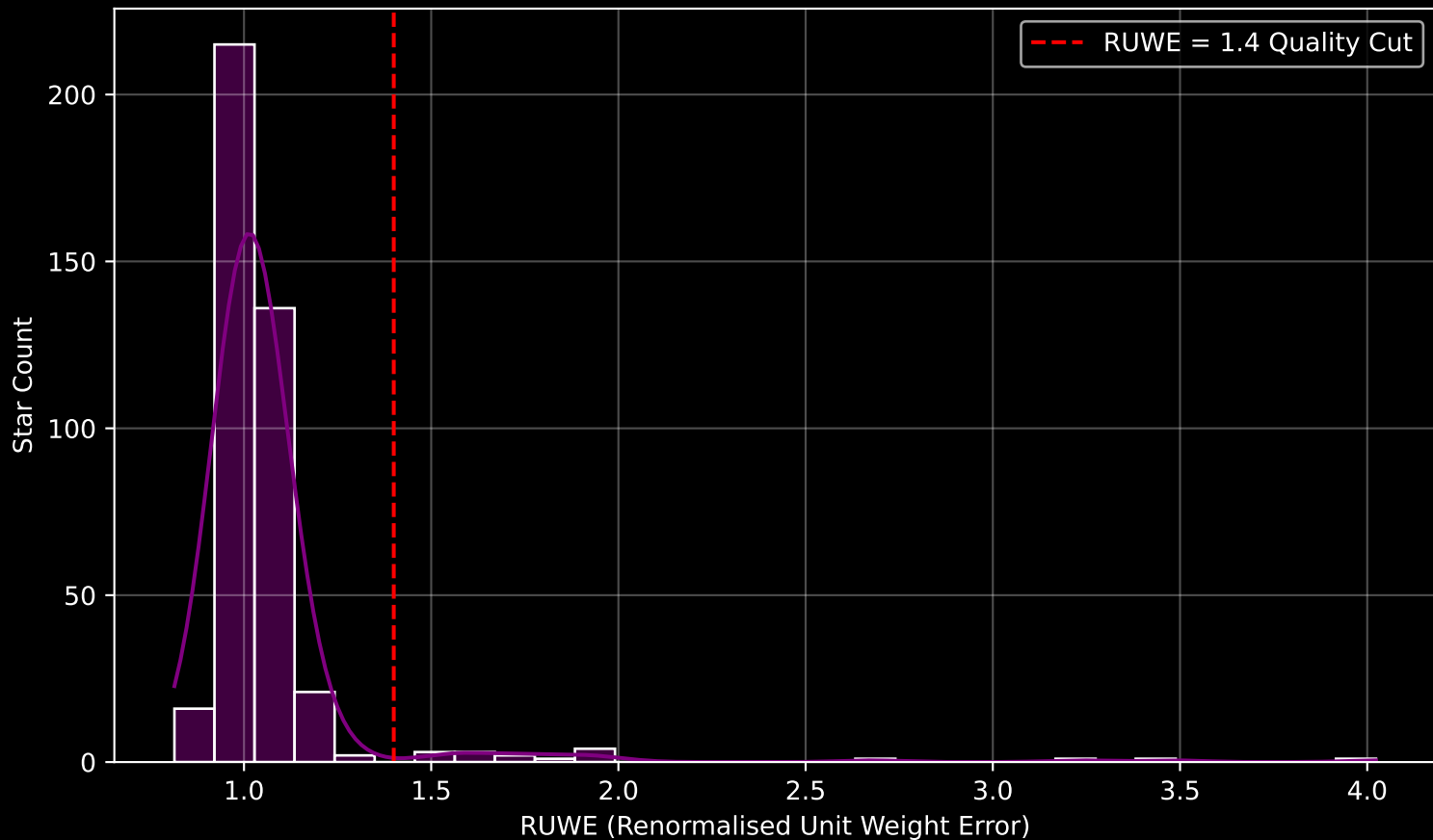
GAPOGEE DR17 Field [281+00] RUWE Distribution (n= 407)
