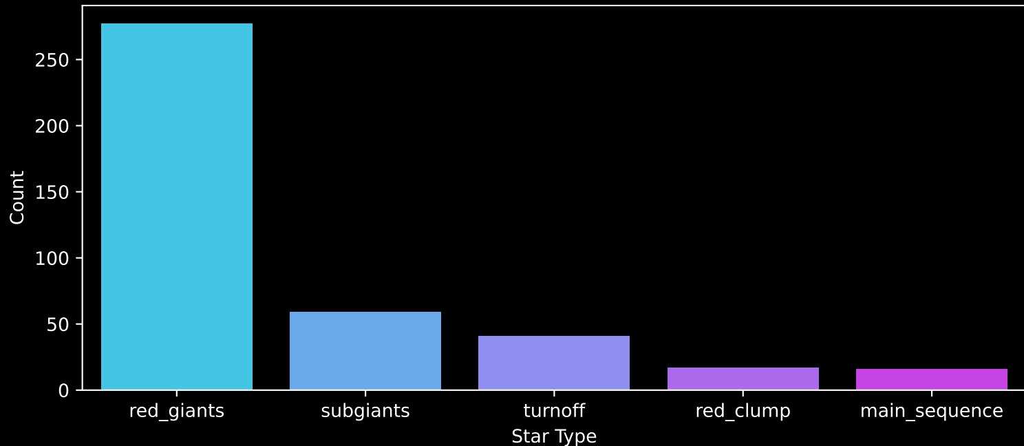
APOGEE DR17 Field: [281+00] Count plot of Star Type
