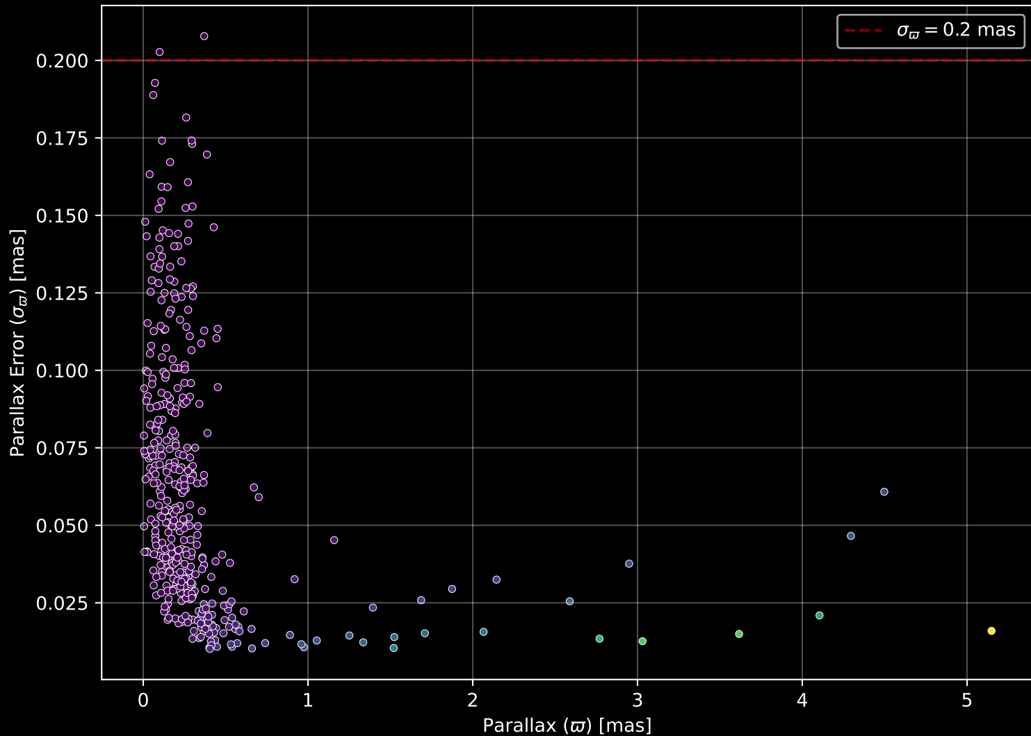
APOGEE DR17 Field: [281+00] Parallax Quality (n= 410)
