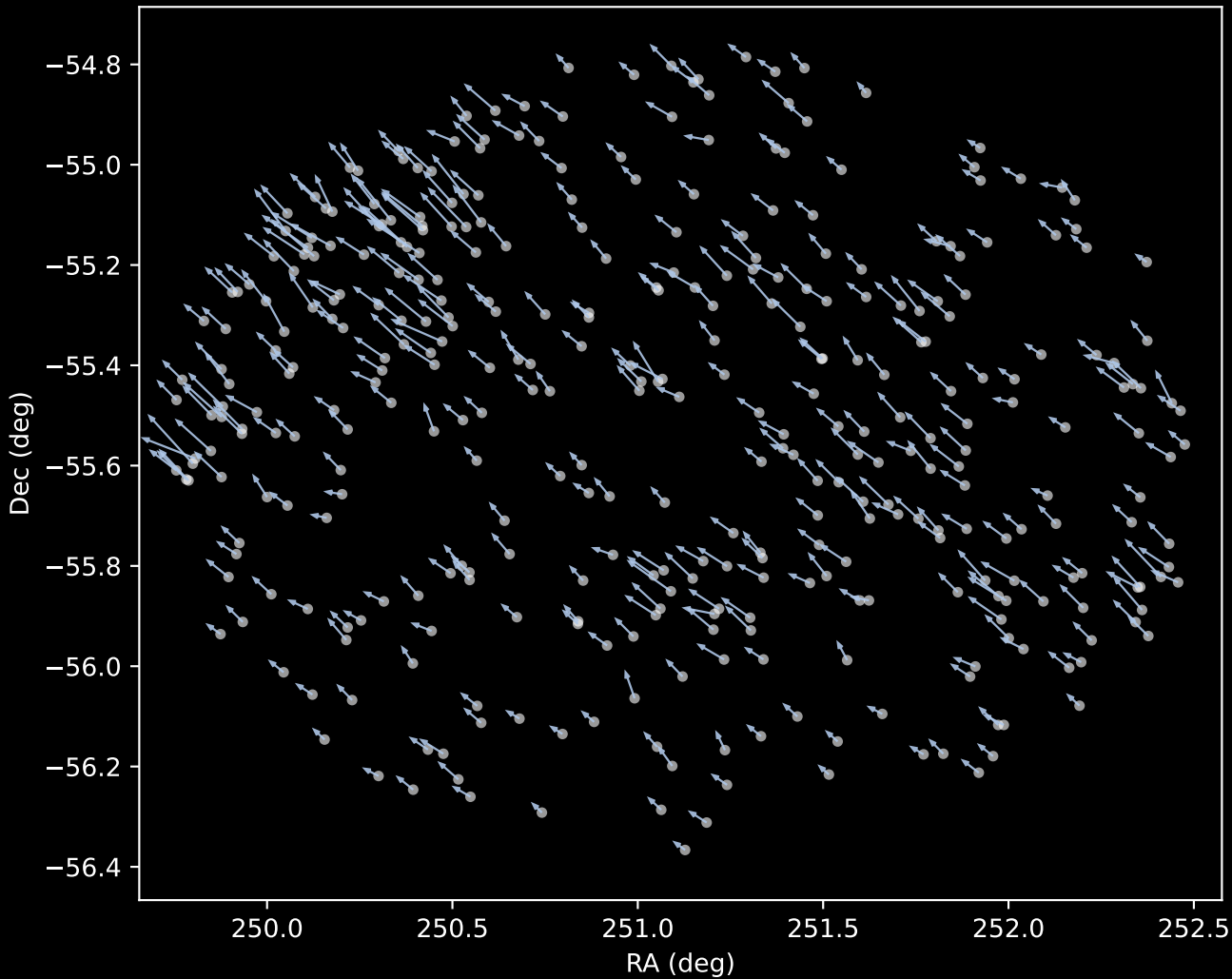
APOGEE DR17 Cluster 1 Proper Motion Vectors (n=369)
